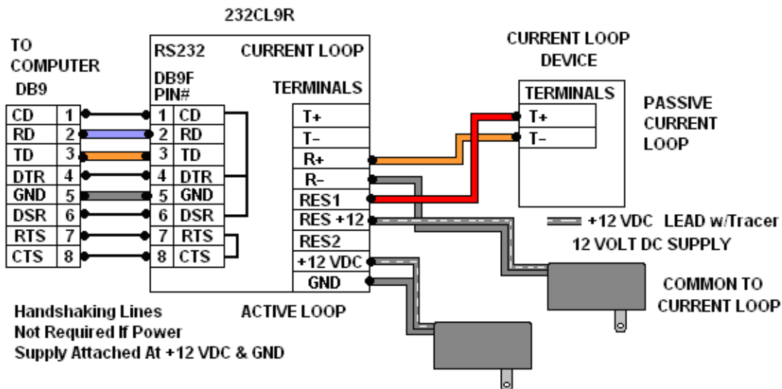
Fig. 7: 232CL9R Active Converter – Passive Device
